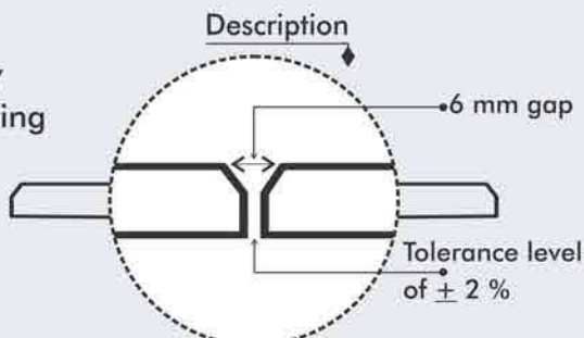
Cross-section of tile after installation
